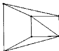
Fig. 5. The reference net.
