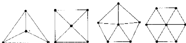
Fig. 8. The first few low-order wheels.
