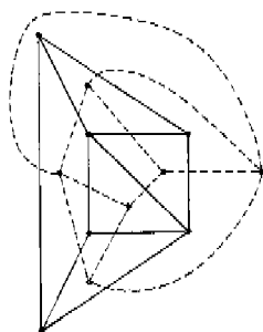
Fig. 6. The reference net and its dual.
