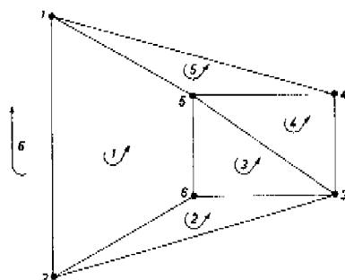
Fig. 7. The reference net.
